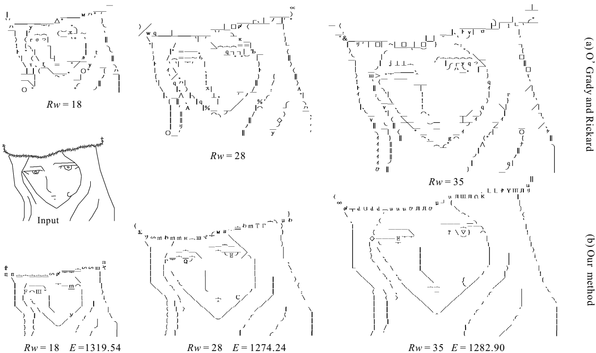
Figure 12: Our method vs. the method of O'Grady and Rickard. R_w is the width of the text resolution and E is the optimized energy.
