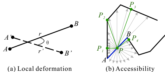
Figure 8: Deformation metric
